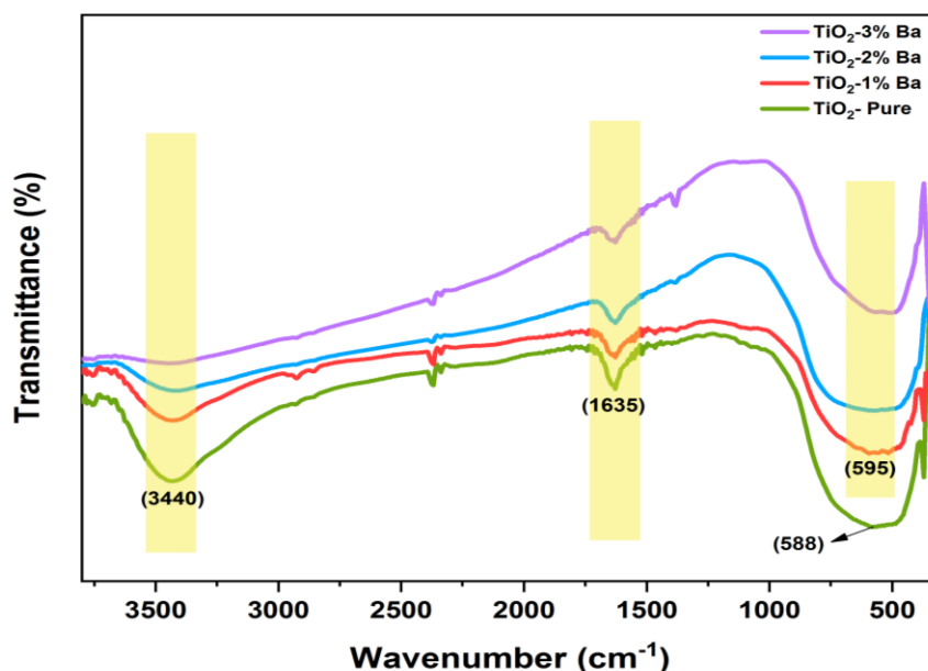
Figure 4. FTIR spectra of pure \text{TiO}_2 and Ba doped \text{TiO}_2
