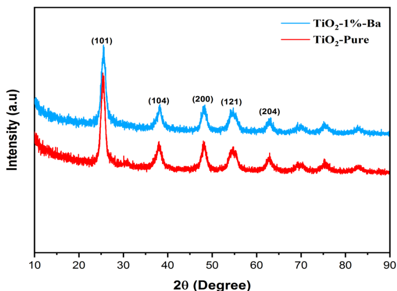
Figure 5. XRD diffractogram of pure \text{TiO}_2 and Ba doped \text{TiO}_2
