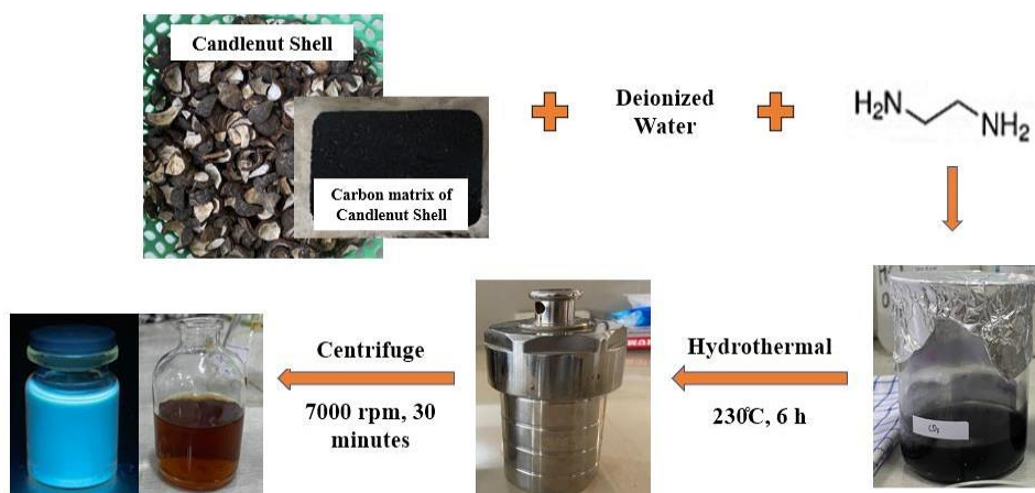
Figure 1. Schematic illustration of the synthesis Carbon Dots
