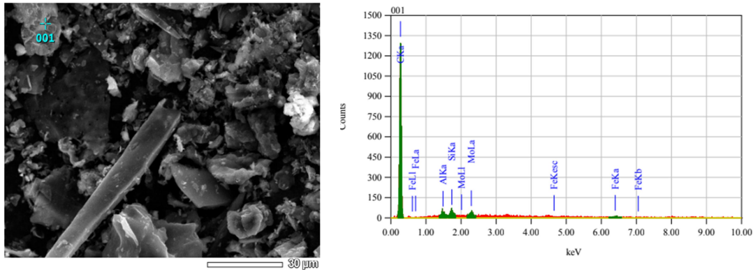
Figure 8. Characterization SEM test results of hybrid briquettes from BFD and coconut shell charcoal composition 60% : 40%.
