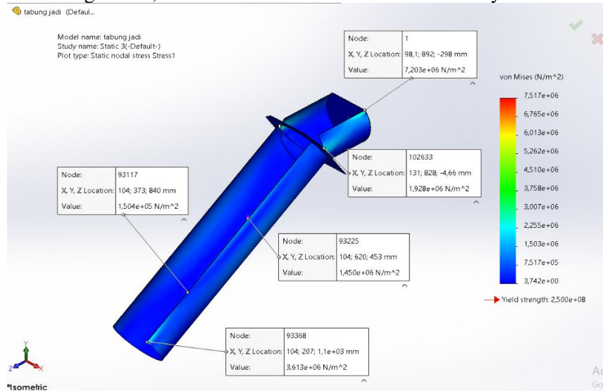
Figure 8. Stress simulation results under a load of 55.154 N.
