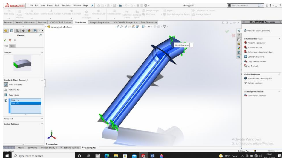
Figure 5. Selection of Support Areas on the Turbine Casing.
